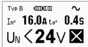
Figure 3.2: Voltage < 24\text{ V} (detailed representation)
