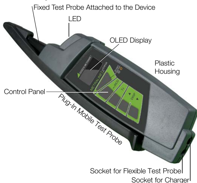
Figure 2.1: Top View
