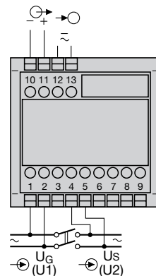
Fig. 4. Power supply connected to the low tension to terminals 12 and 13.
