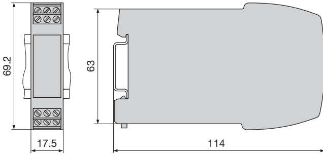
Fig. 8. SINEAX TV 809 in carrying rail housing P12/17 clipped onto a top-hat rail (35 x 15 mm or 35 x 7.5 mm, acc. to EN 50 022), screw terminals not pluggable .
