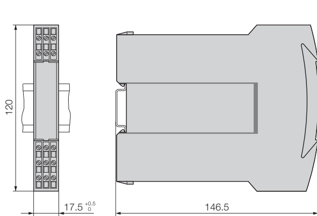
Fig. 3. SINEAX TV 808 in housing S17 clipped onto a top-hat rail (35x15 mm or 35x7.5 mm, acc. to EN 50 022).
