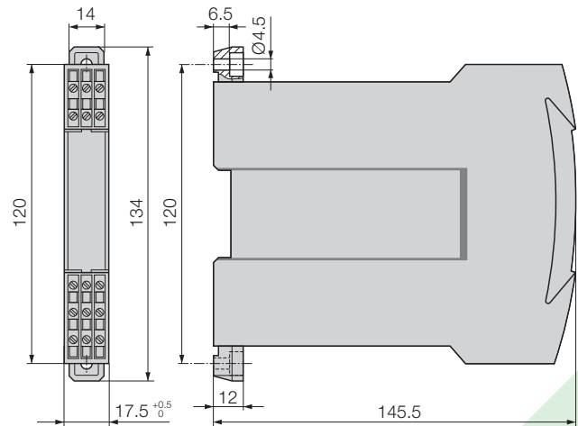
Fig. 4. SINEAX TV 808 in housing S1 , screw hole mounting brackets pulled out.
