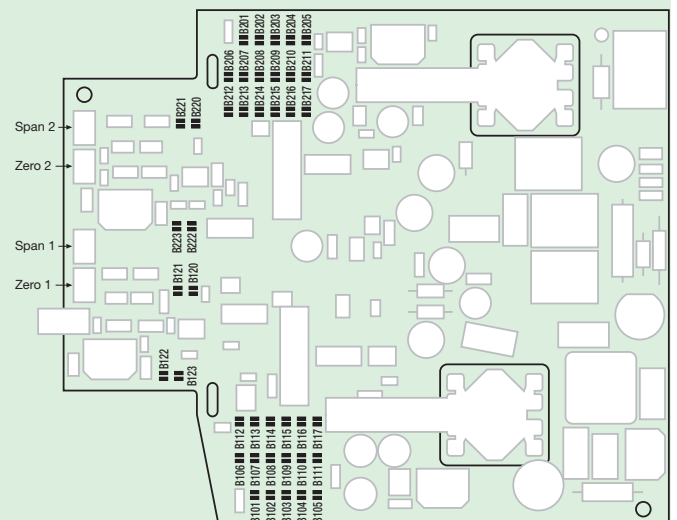
Fig. 2. Position of the soldered jumpers B ... and the potentiometers "Span" and "Zero".
