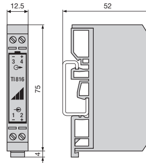
Fig. 9. SINEAX TI 816 on G-type rail EN 50 035 – G 32.
