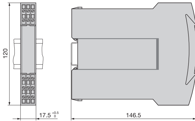
Fig. 16. SINEAX B 811 in housing S17 clipped onto a top-hat rail (35 x 15 mm or 35 x 7.5 mm, acc. to EN 50 022).
